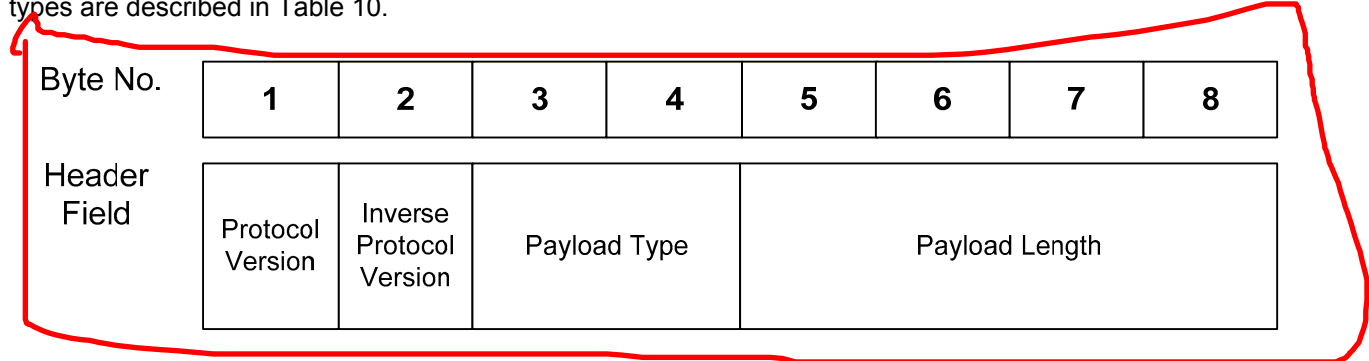
Figure 9 — V2GTP Message header structure
