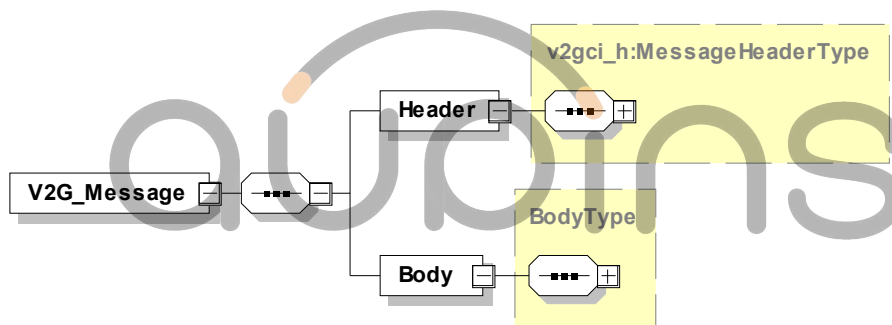
Figure 19 — Schema Diagram – V2G message
